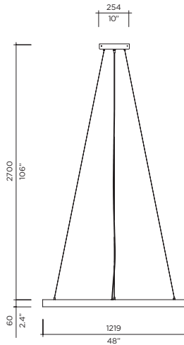
Model Ring Suspension Size 1219 Ref. # GM.07.500._._ Lamping 1 x 48w LED 3000K, 3840Lm LED E
