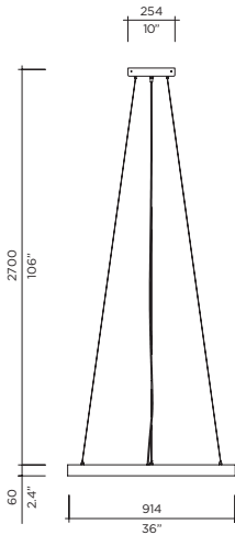
Model Ring Suspension Size 914 Ref. # MM.07.500._._ Lamping 1 x 36w LED 3000K, 2880Lm LED E
