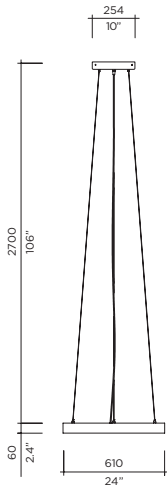
Model Ring Suspension Size 610 Ref. # SM.07.500._._ Lamping 1 x 30W LED 3000K, 2400Lm LED E
