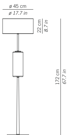
LSH11 --- Lampada da terra Floor lamp 1xE27 105W HS CE IP20 □
