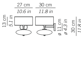
LSH23 --- Lampada da parete Wall lamp 1xE27 70W HS CE IP20
