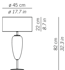
LSH06 --- Lampada da tavolo grande Large table lamp 1xE27 105W HS CE IP20 □
