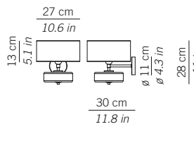
LSH24 --- Lampada da parete Wall lamp 1xE27 70W HS CE IP20
