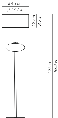
LSH13 --- Lampada da terra Floor lamp 1xE27 105W HS CE IP20 □
