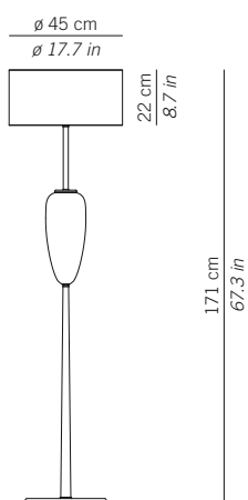
LSH12 --- Lampada da terra Floor lamp 1xE27 105W HS CE IP20 □
