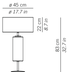
LSH05 --- Lampada da tavolo grande Large table lamp 1xE27 105W HS CE IP20 □
