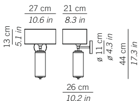
LSH21 --- Lampada da parete Wall lamp 1xE27 70W HS CE IP20
